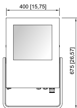
Floodlight without cooling element
