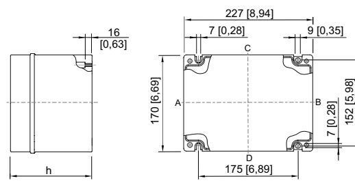
8146/.06. 8146/.061: h = 91 mm [3.58 inch] 8146/.062: h = 131 mm [5.16 inch]
