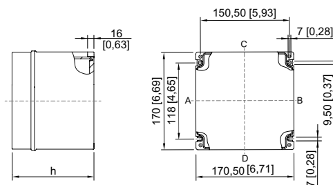
8146/.05. 8146/.051: h = 91 mm [3.58 inch] 8146/.052: h = 131 mm [5.16 inch]
