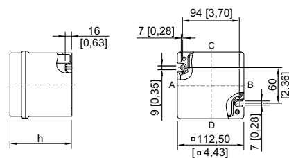
8146/.03. 8146/.031: h = 91 mm [3.58 inch] 8146/.037: h = 104 mm [4.09 inch]
