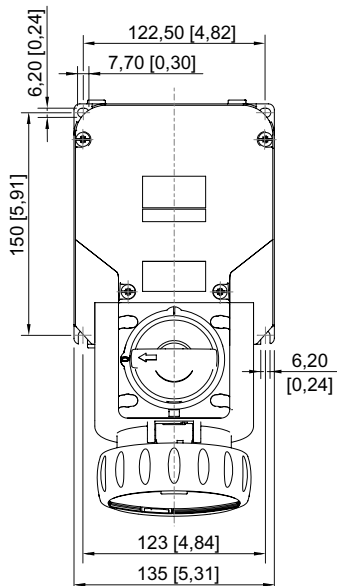
Wall-mounting socket
